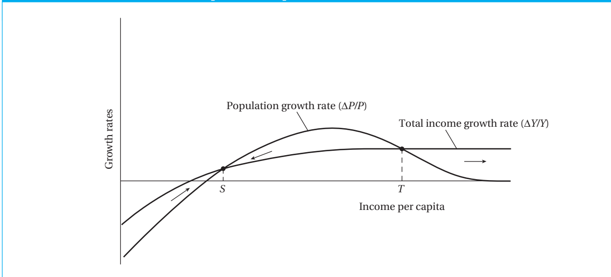
FIGURE 6.7 The Malthusian Population Trap
