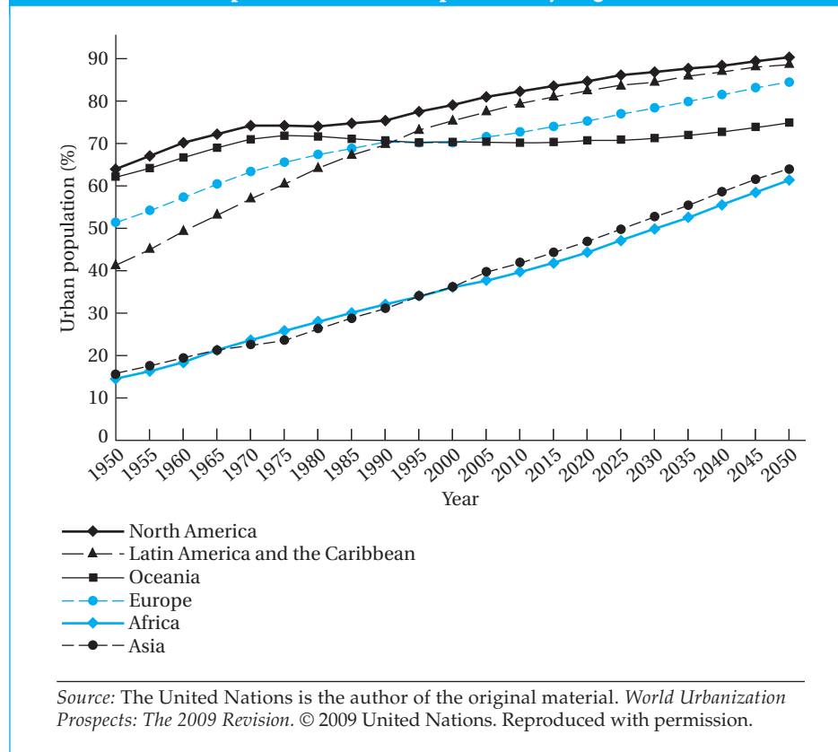
FIGURE 7.3 Proportion of Urban Population by Region, 1950–2050
